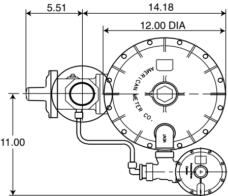
1-1/2" and 2" Model 1883 PFM Pilot Loaded Regulator
