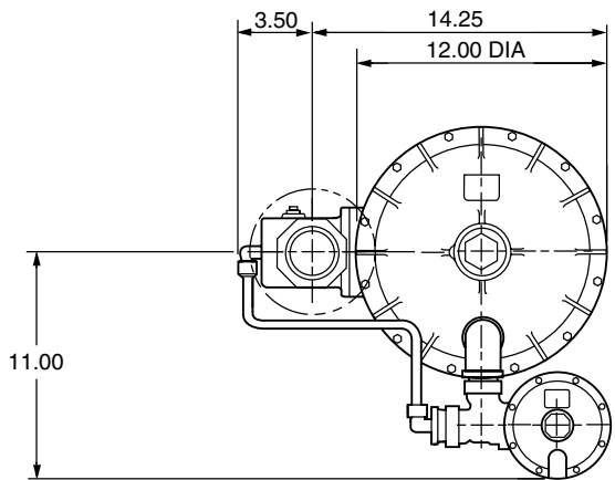
1-1/2" and 2" Model 1803 PFM Pilot Loaded Regulator
