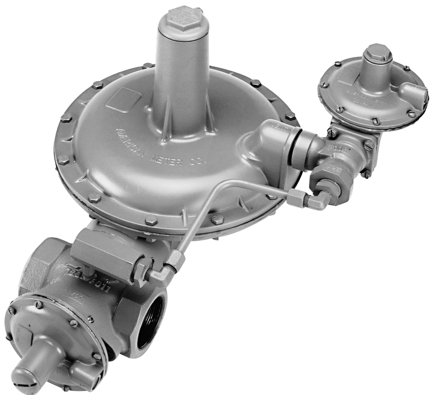
1-1/2" and 2" Model 1803 PFM Pilot Loaded Regulator
