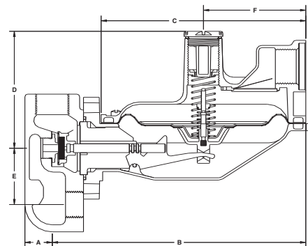
1813B2 - Offset
