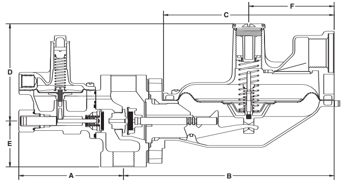
Model 1843B2
