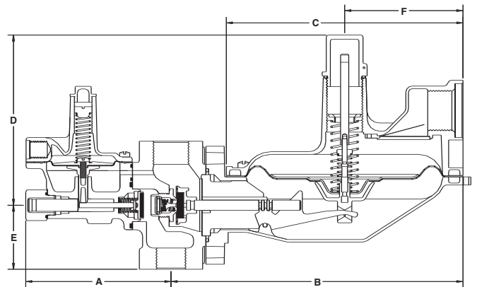
Model 1853B2
